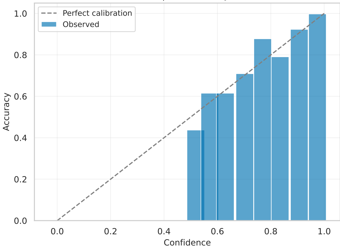
resnet34 | val Reliability (raw)
