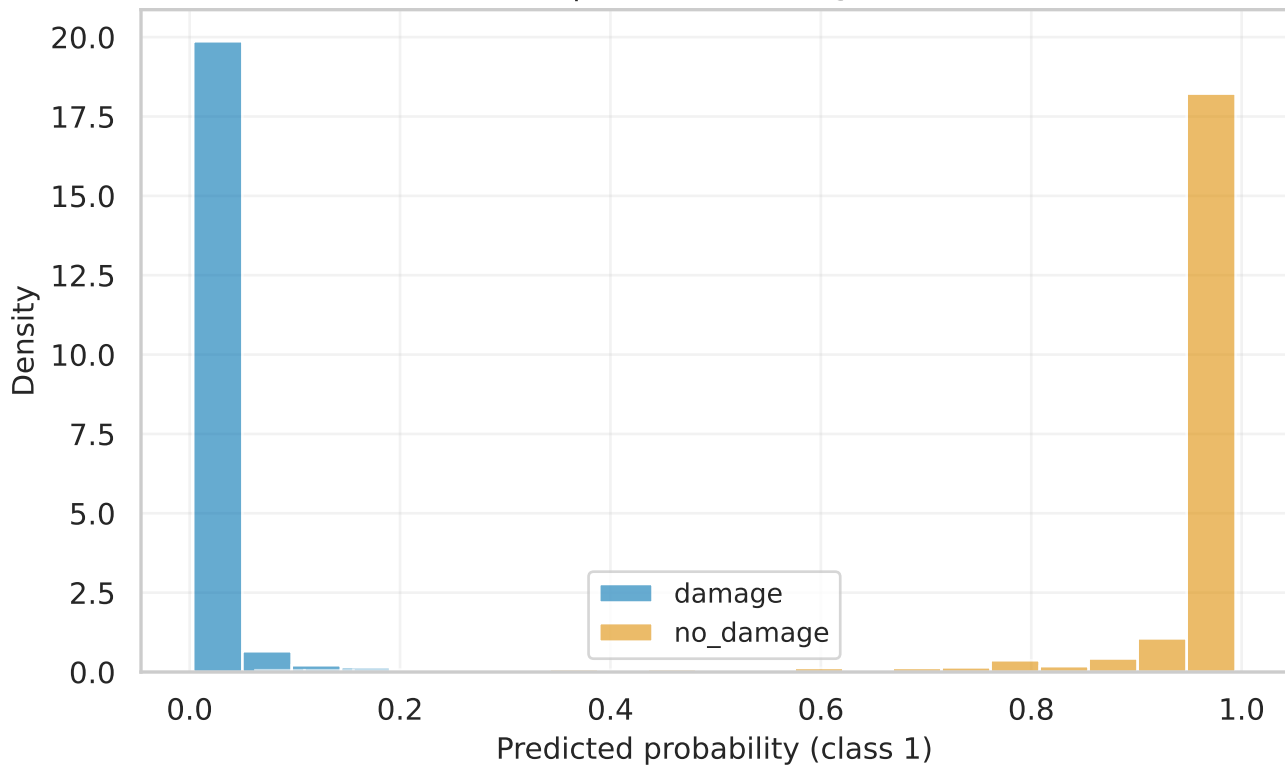
resnet50 | val Score Histogram (raw)
