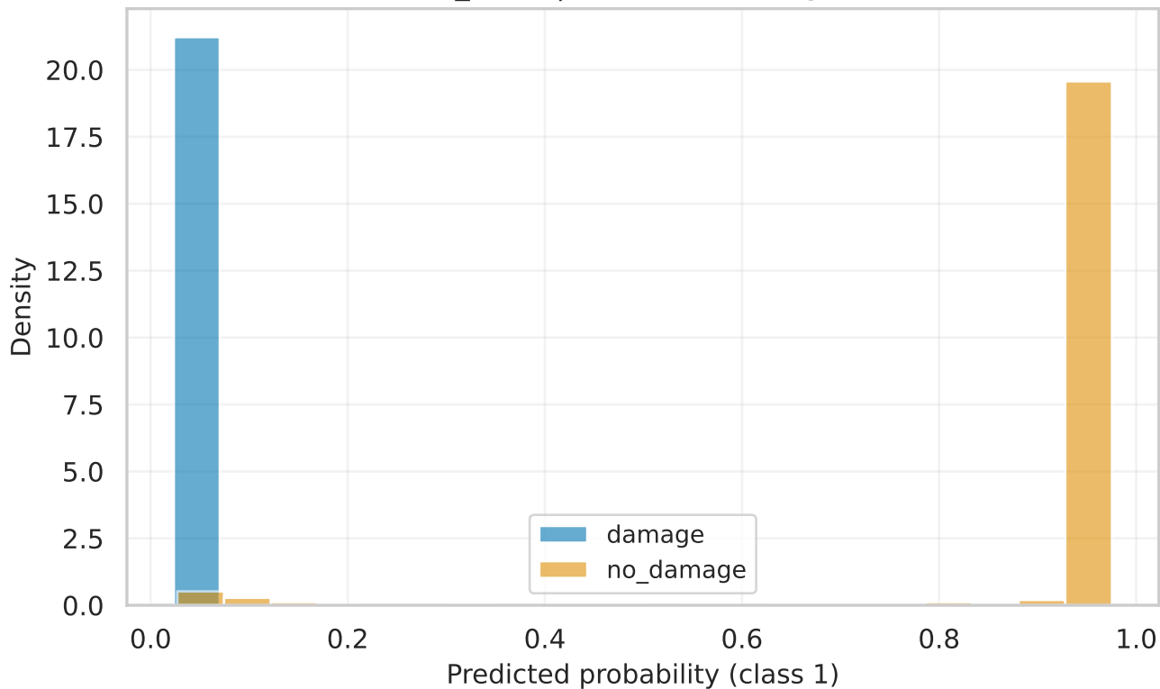
convnext_small | test Score Histogram (raw)
