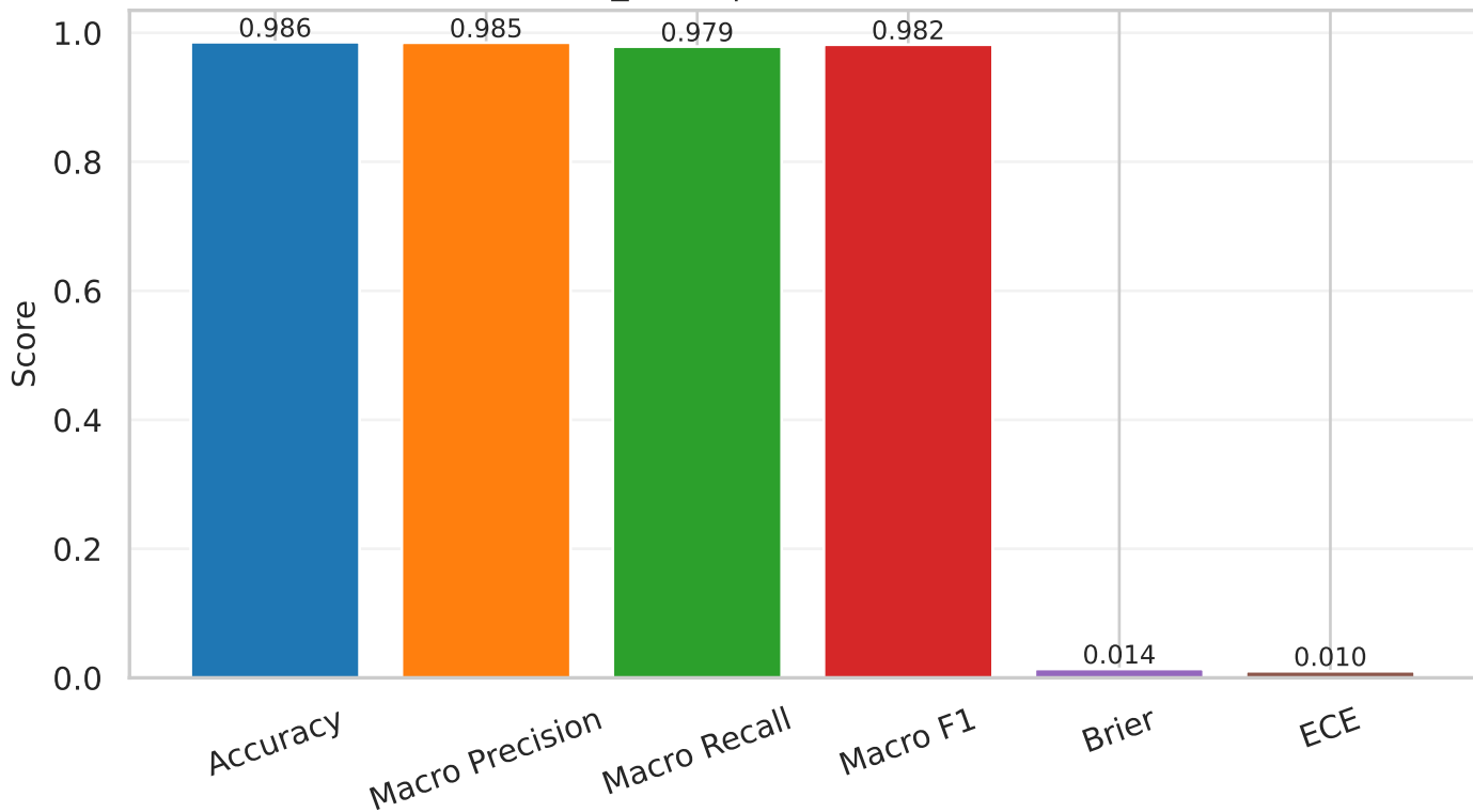
convnext_small | val (calibrated) metrics
