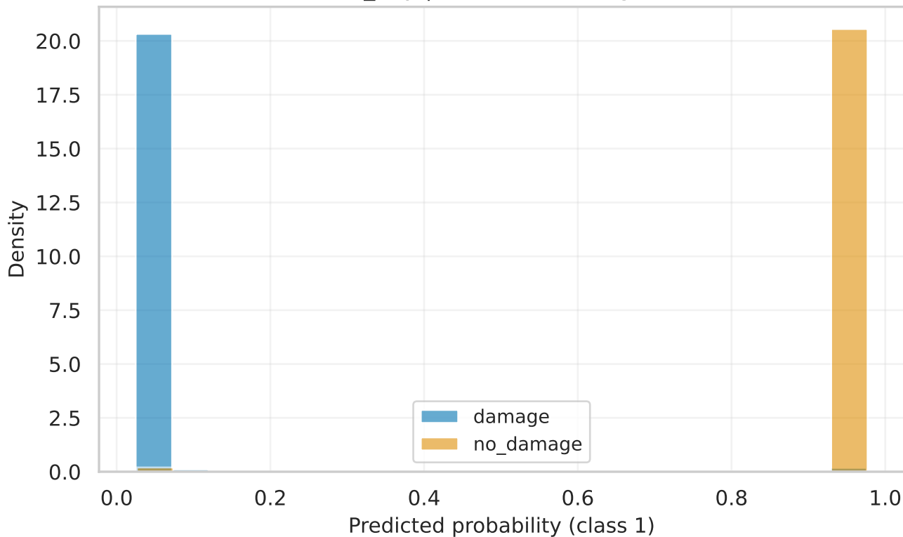
convnext_tiny | test Score Histogram (raw)
