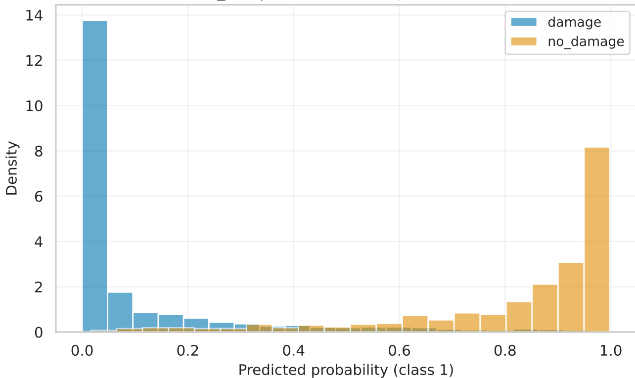
custom_cnn | test Score Histogram (calibrated)
