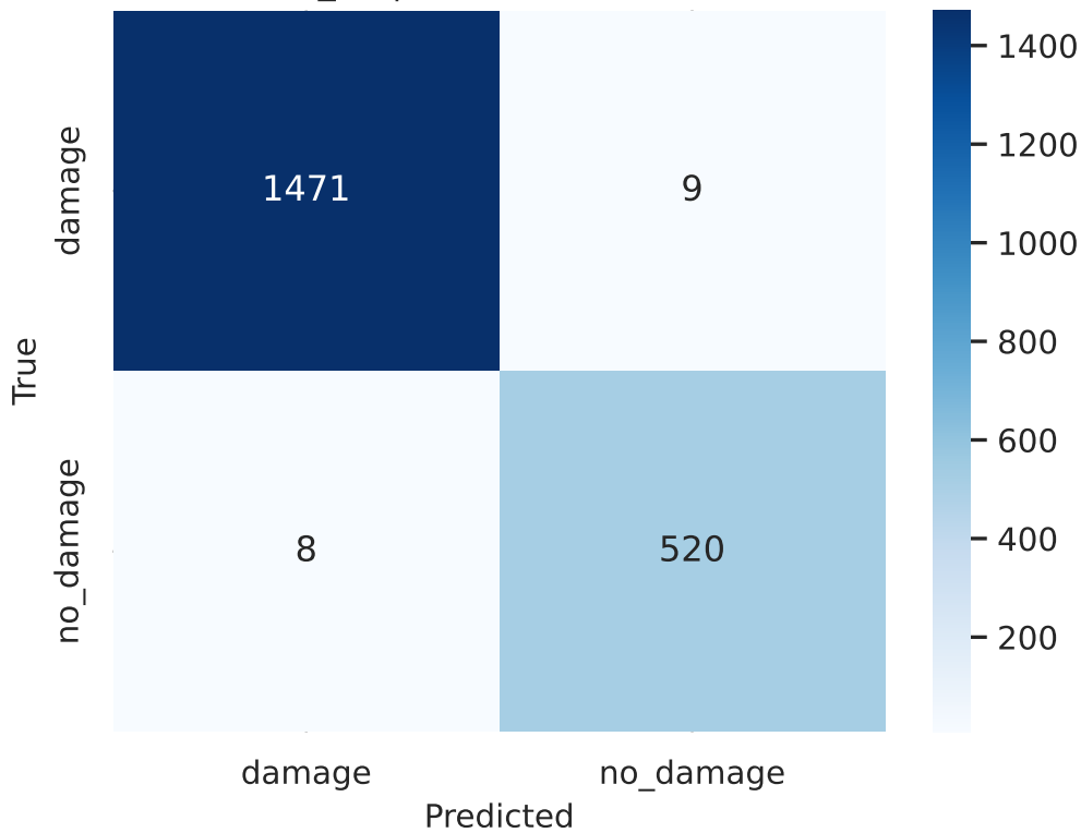
efficientnet_b1 | test Confusion (calibrated)
