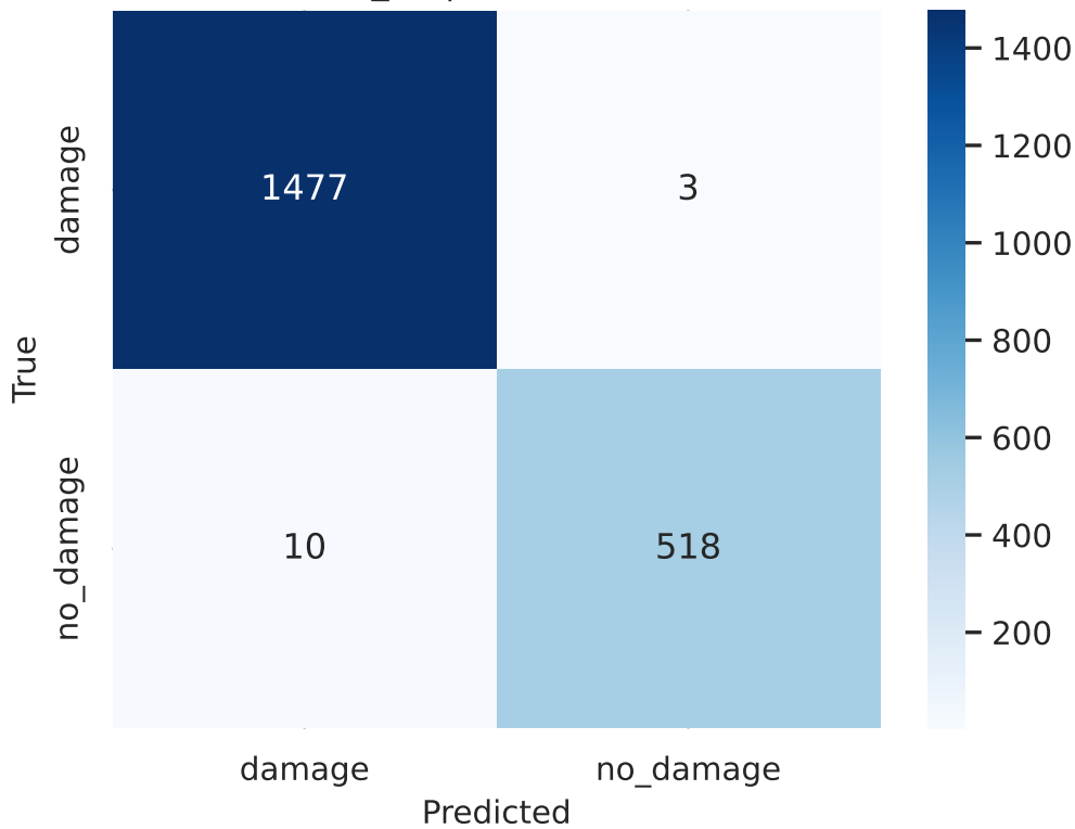
efficientnet_b2 | test Confusion (raw)
