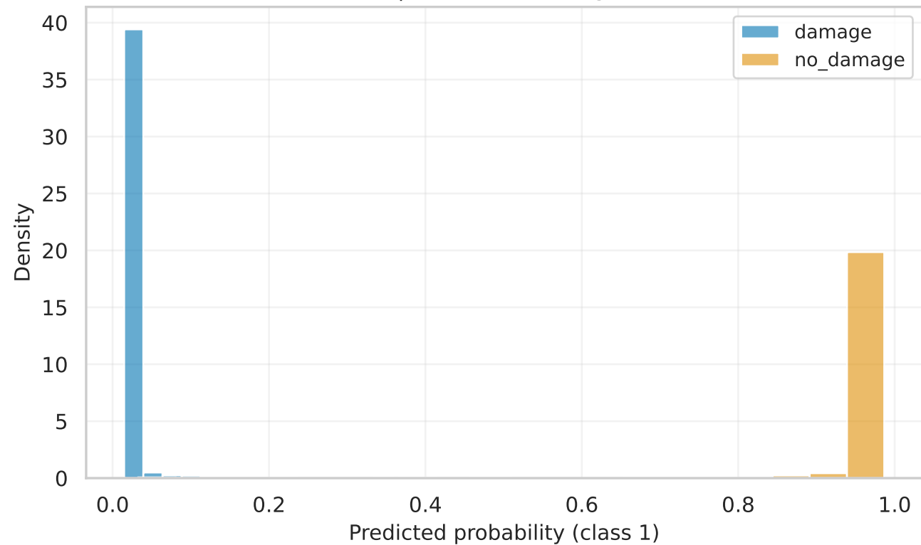
resnet18 | test Score Histogram (raw)
