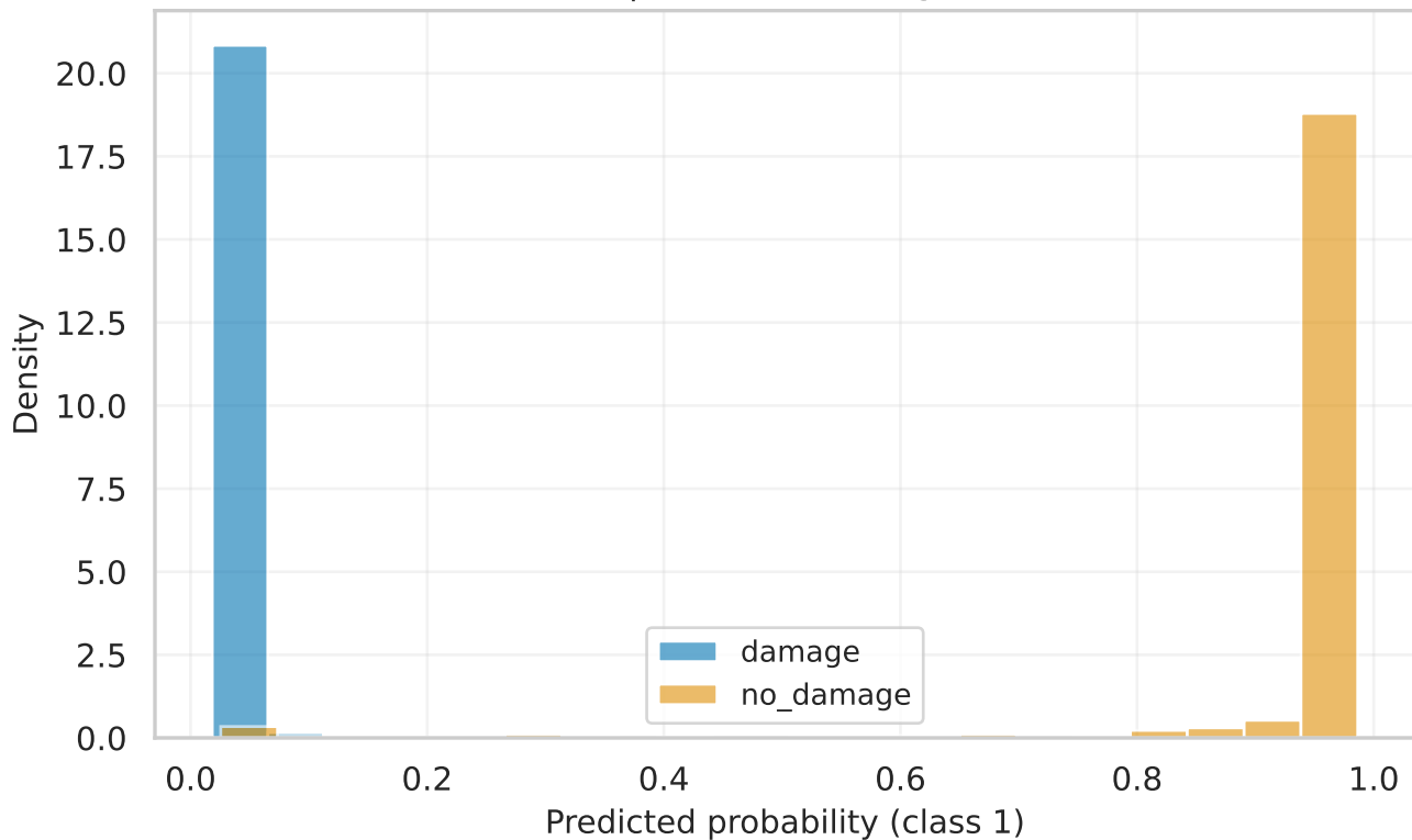
resnet18 | val Score Histogram (raw)
