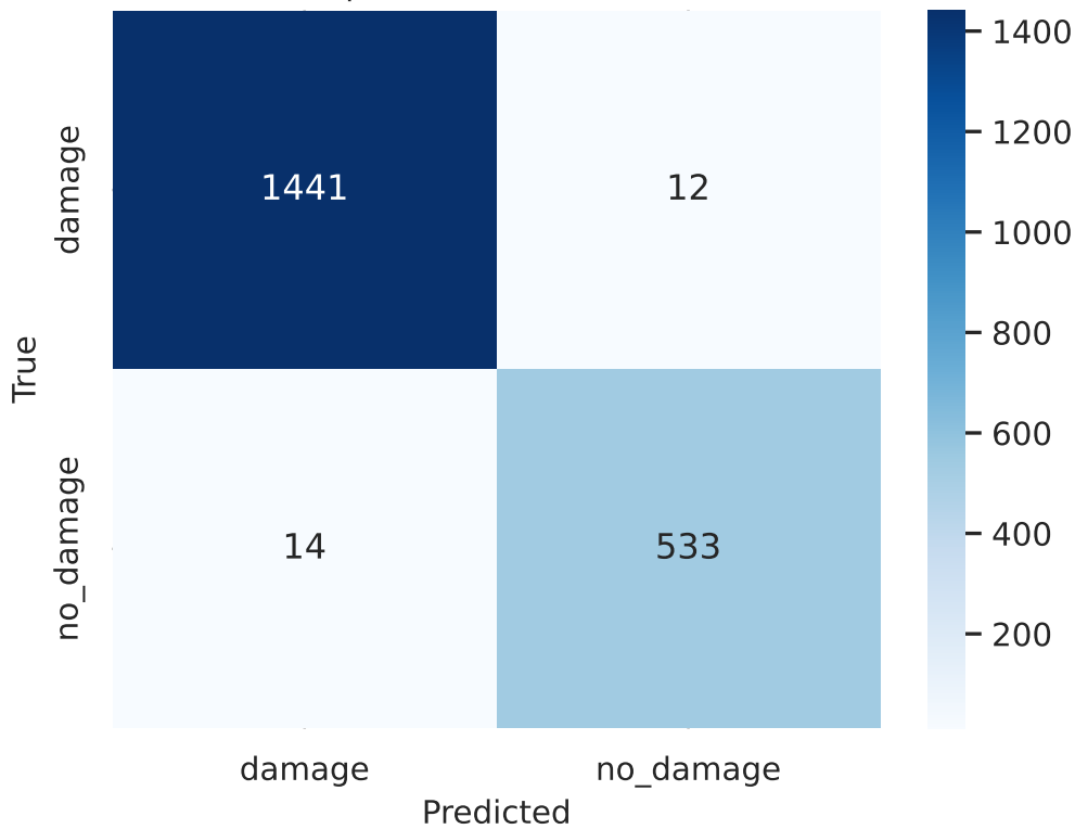
resnet34 | val Confusion (calibrated)
