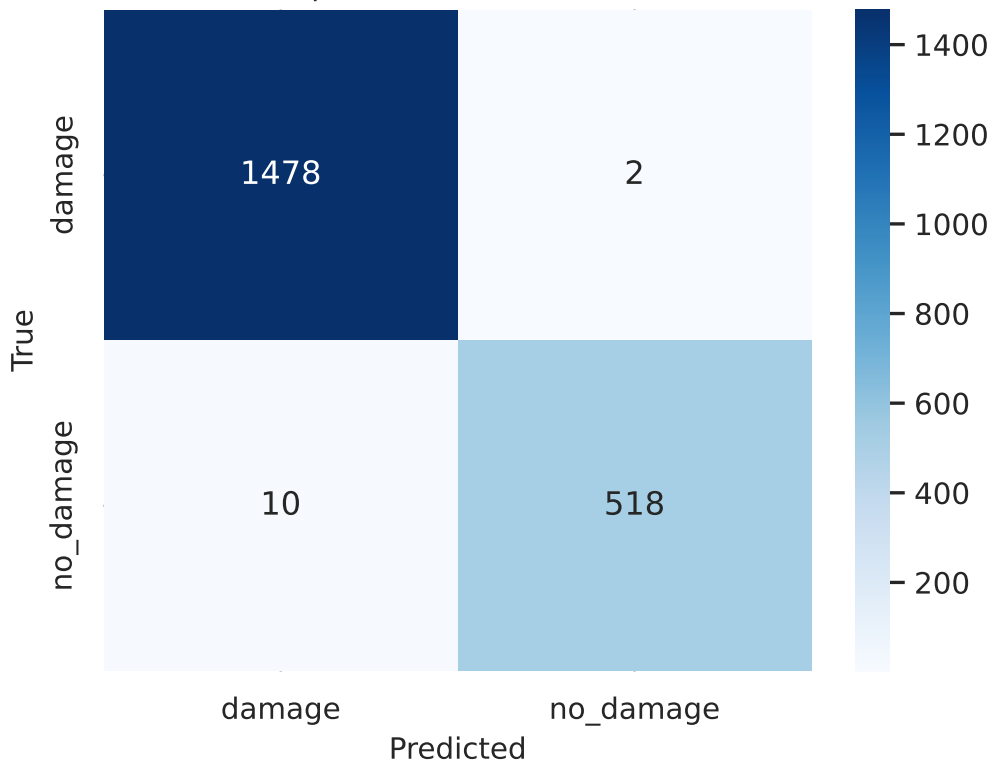
resnet50 | test Confusion (calibrated)
