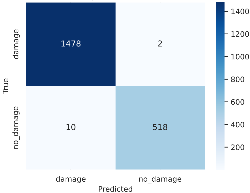
resnet50 | test Confusion (raw)
