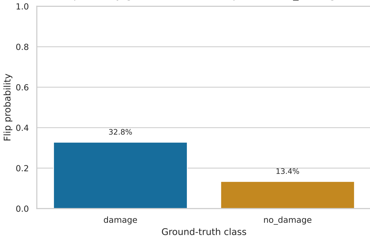
Flip rate by ground-truth class (profile->no_damage)
