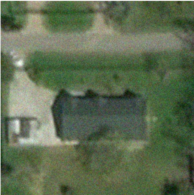
validation/no_damage,validation_no_damage_-95.196208_29.537188_1a1a1a.jpeg,validation_no_damage_-96.936996_28.768817_72e9d.jpg,validation_no_damage_-96.947272_28.810505_aa3d3b.jpeg
