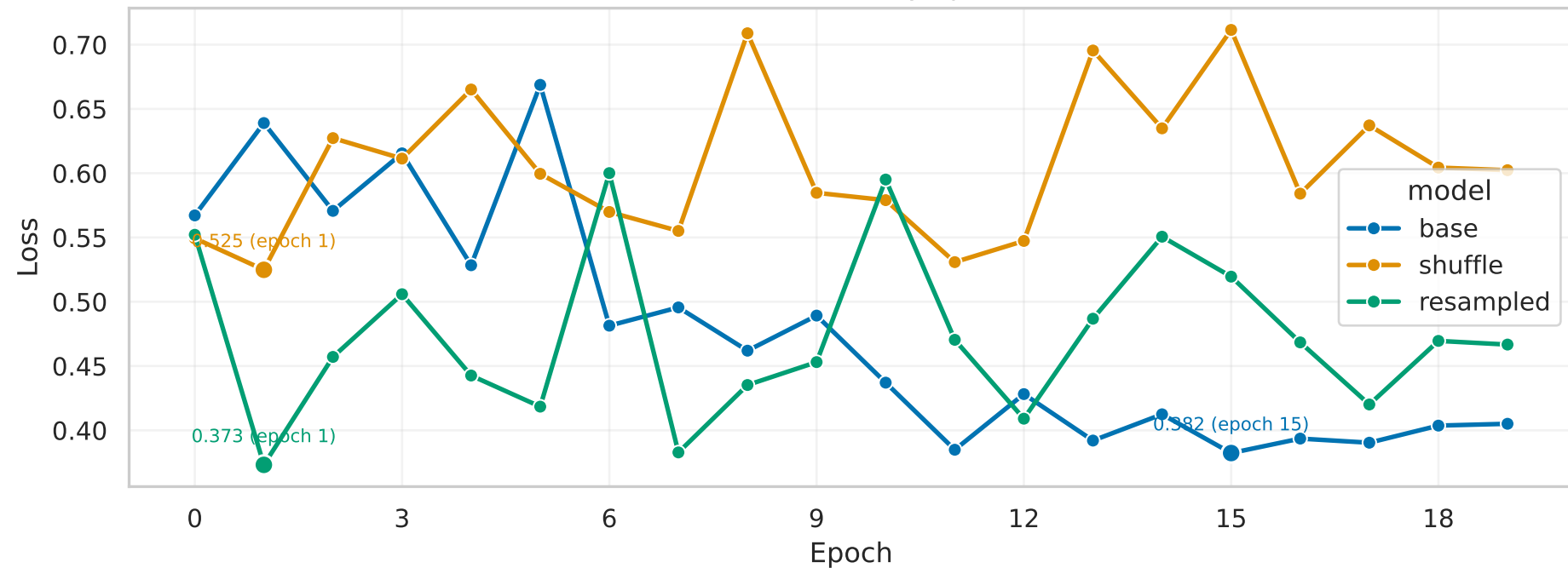
Validation loss by epoch
