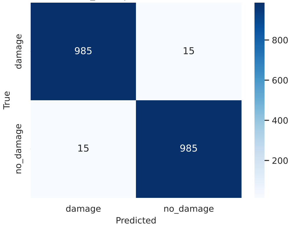
convnext_small | test Confusion (raw)
