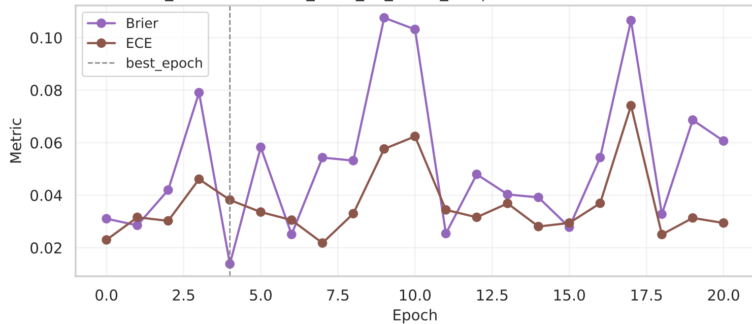
convnext_small (Run: data_2025_12_11-22_35) | Calibration metrics (Brier/ECE)
