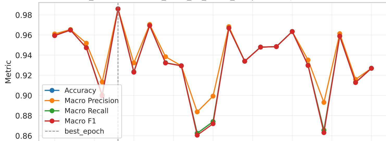
convnext_small (Run: data_2025_12_11-22_35) | Accuracy/Precision/Recall/F1
