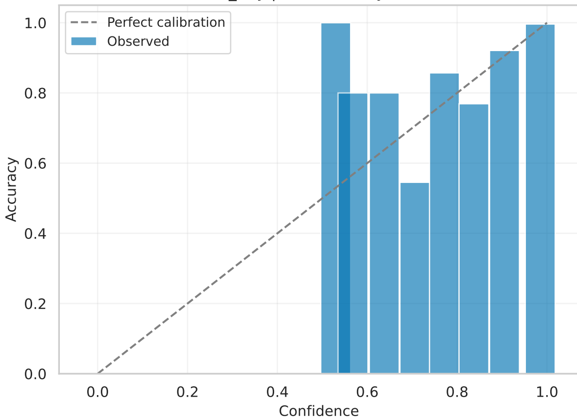
convnext_tiny | val Reliability (calibrated)
