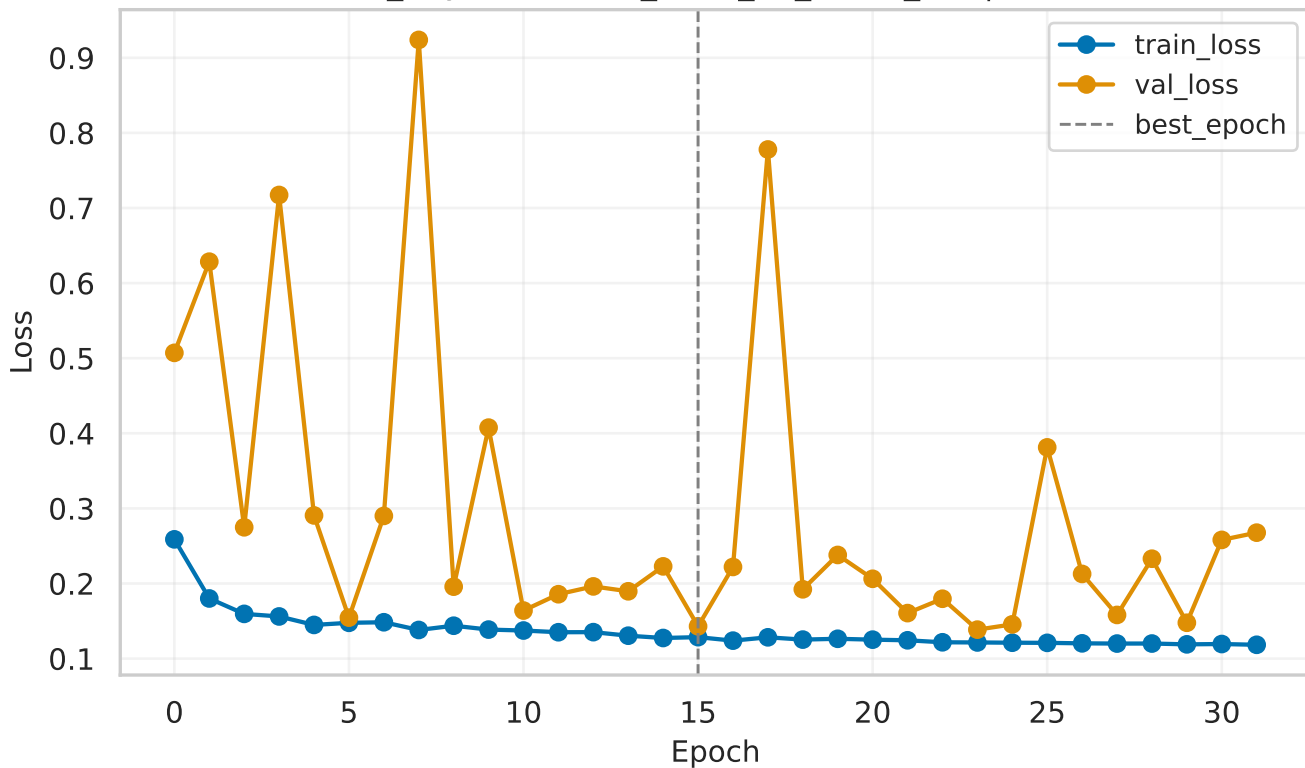
convnext_tiny (Run: data_2025_12_11-22_35) | Loss curves
