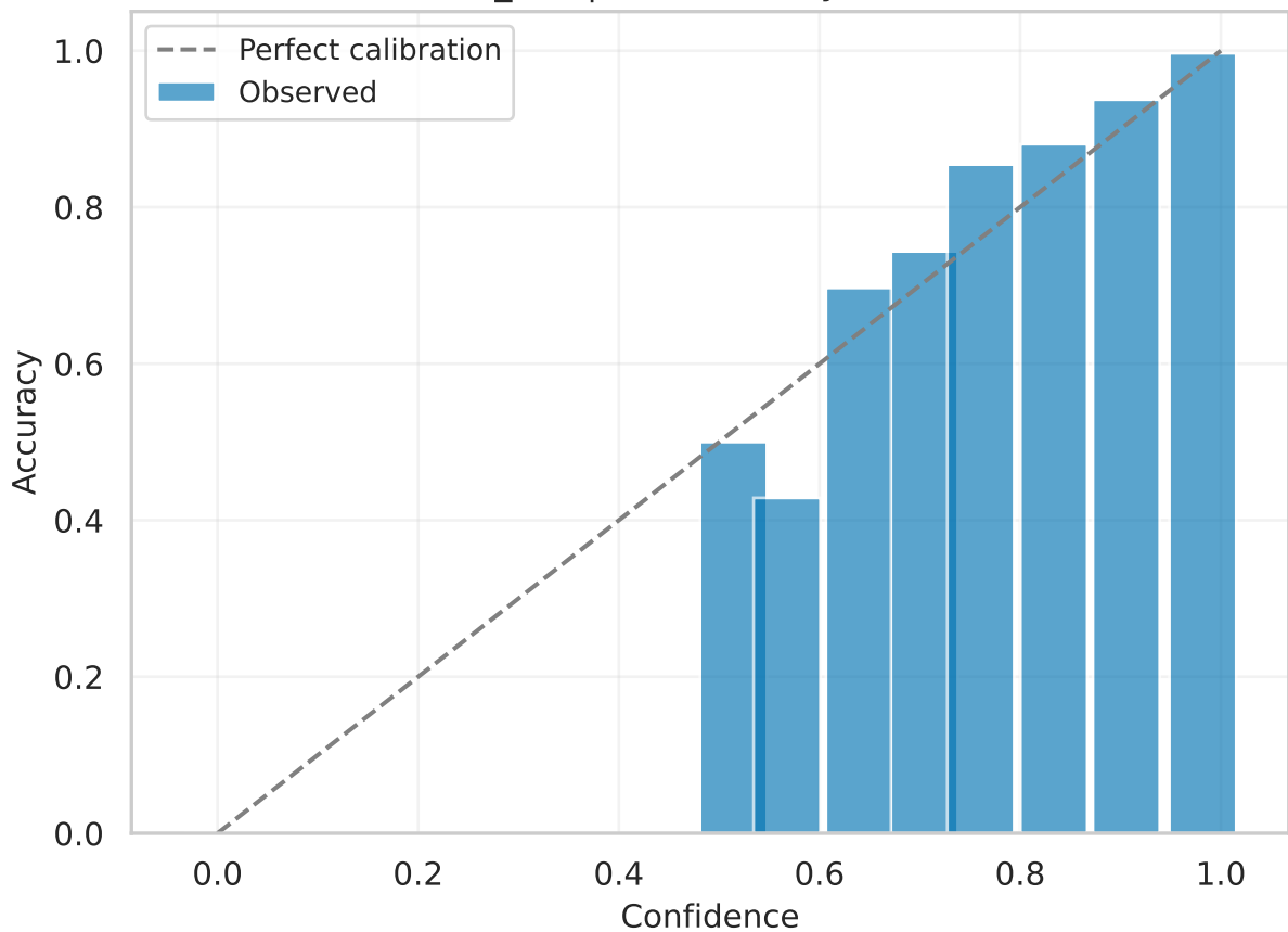
custom_cnn | val Reliability (calibrated)
