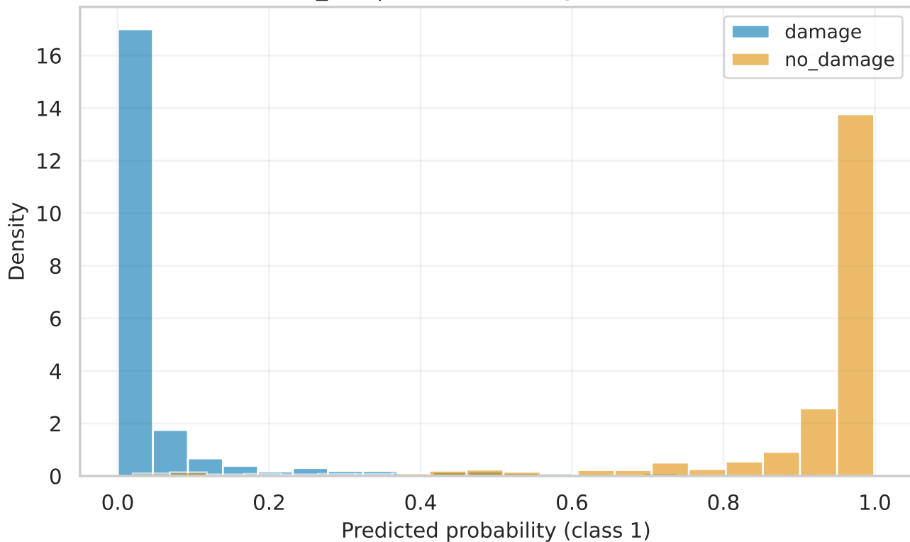
custom_cnn | val Score Histogram (calibrated)
