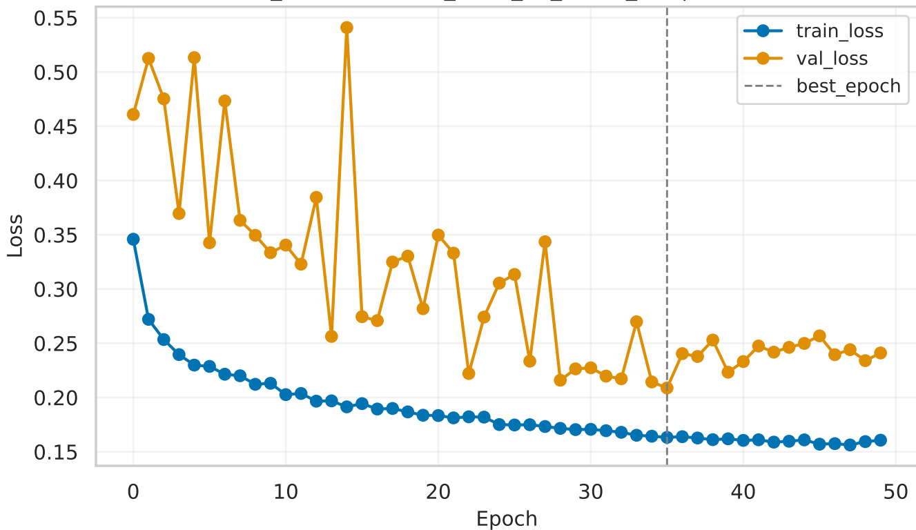
custom_cnn (Run: data_2025_12_11-22_35) | Loss curves
