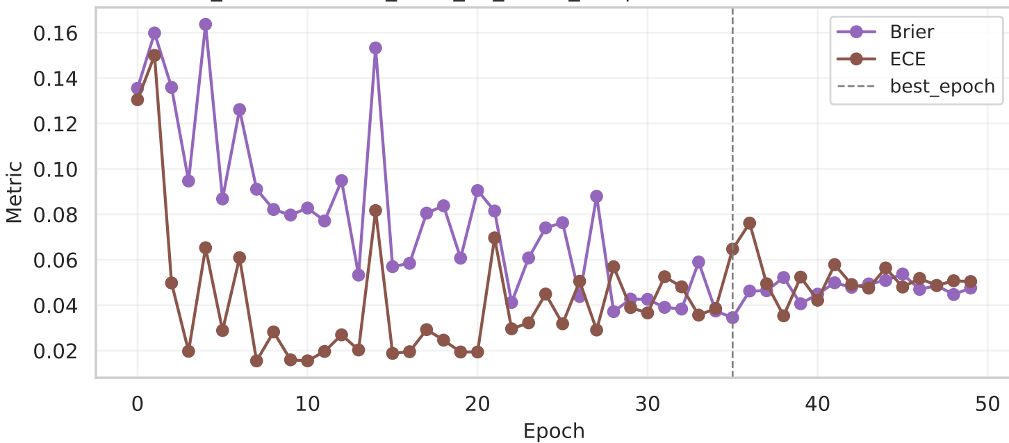
custom_cnn (Run: data_2025_12_11-22_35) | Calibration metrics (Brier/ECE)
