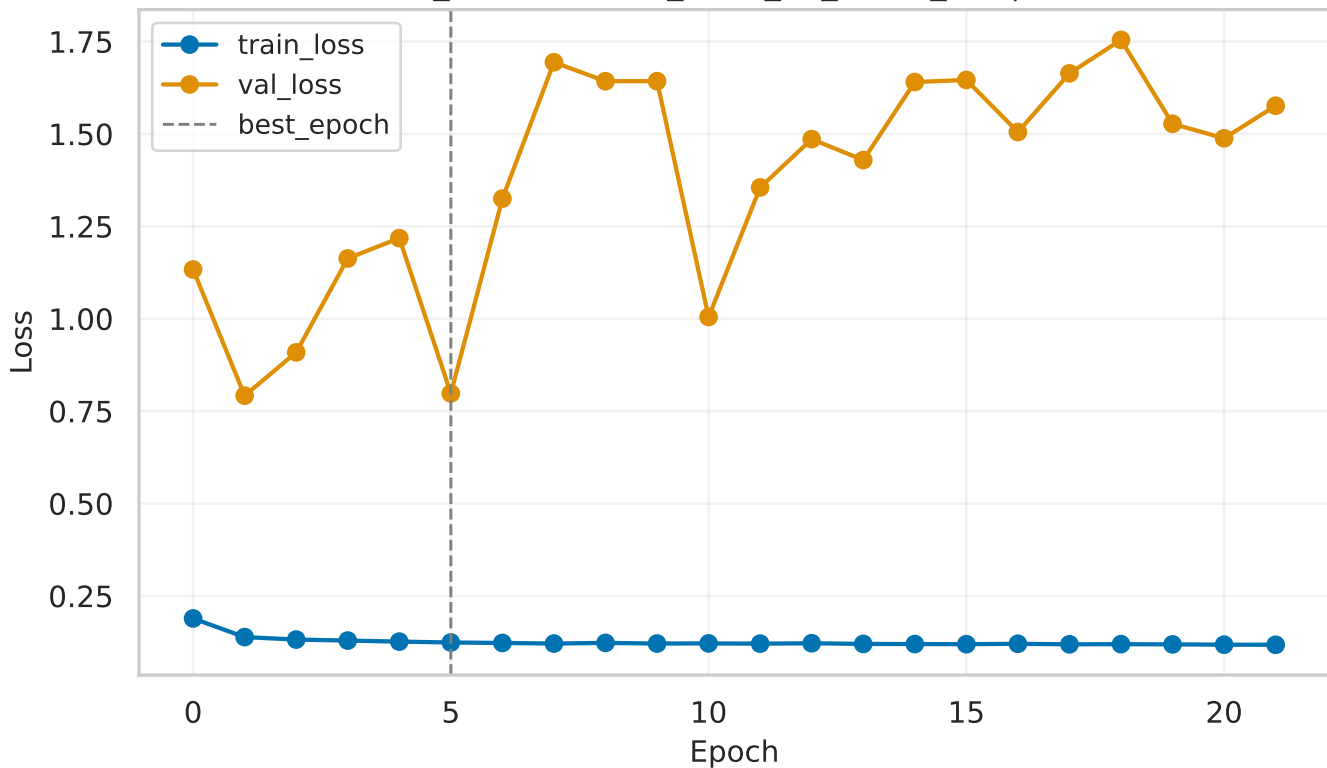
efficientnet_b1 (Run: data_2025_12_11-22_35) | Loss curves
