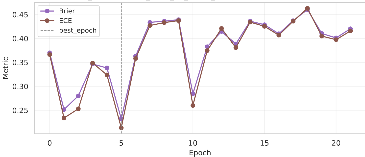
efficientnet_b1 (Run: data_2025_12_11-22_35) | Calibration metrics (Brier/ECE)
