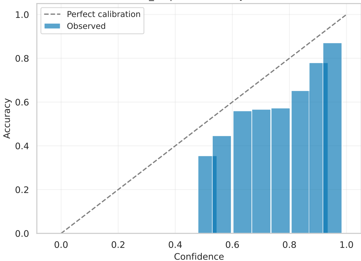
efficientnet_b2 | test Reliability (calibrated)
