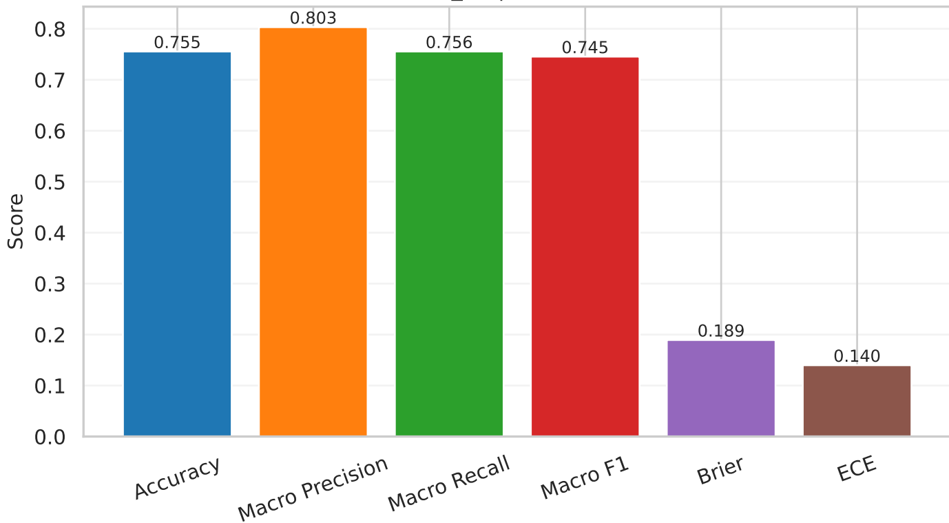
efficientnet_b2 | test (raw) metrics
