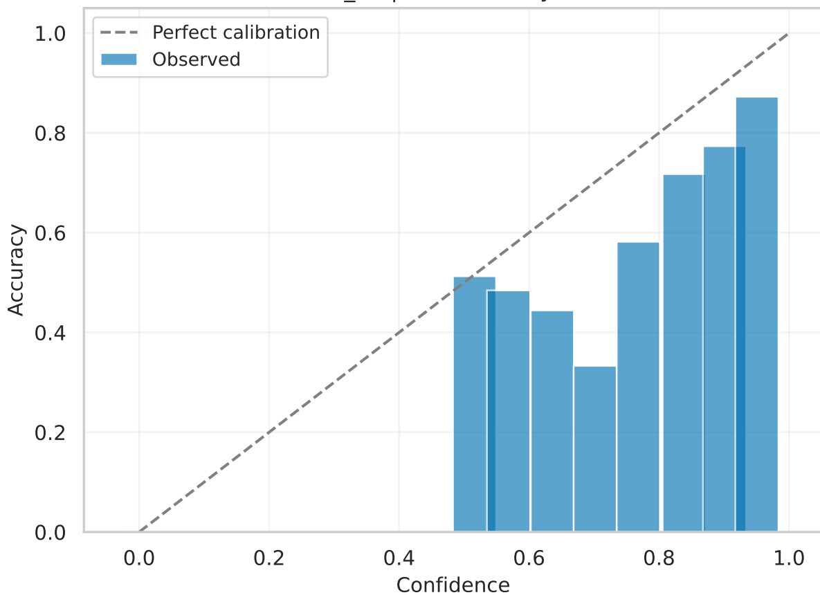
efficientnet_b2 | val Reliability (calibrated)
