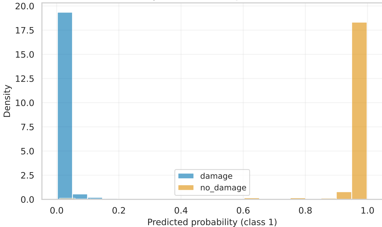
resnet18 | test Score Histogram (calibrated)
