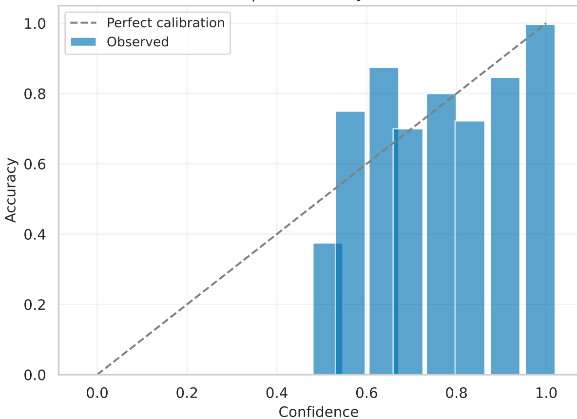
resnet18 | val Reliability (calibrated)
