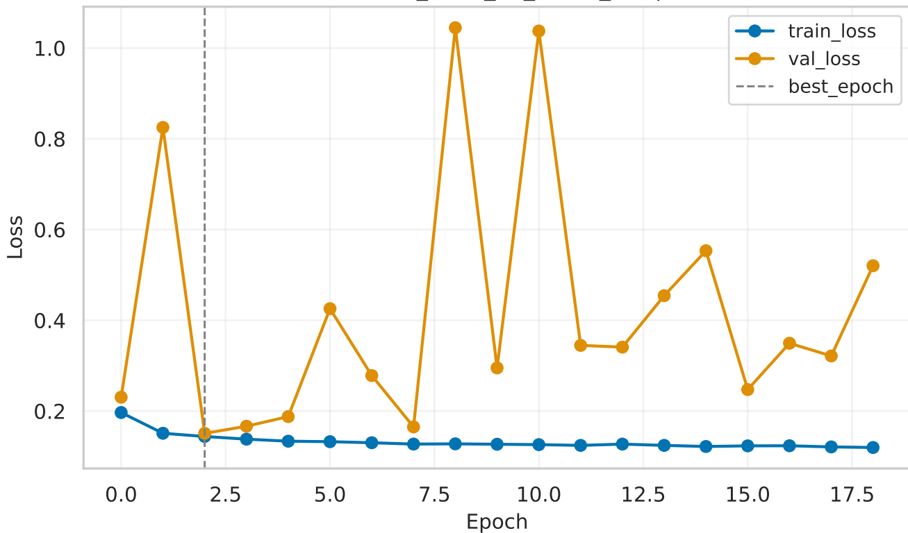
resnet18 (Run: data_2025_12_11-22_35) | Loss curves
