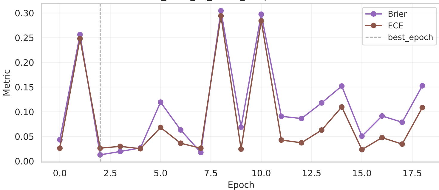
resnet18 (Run: data_2025_12_11-22_35) | Calibration metrics (Brier/ECE)
