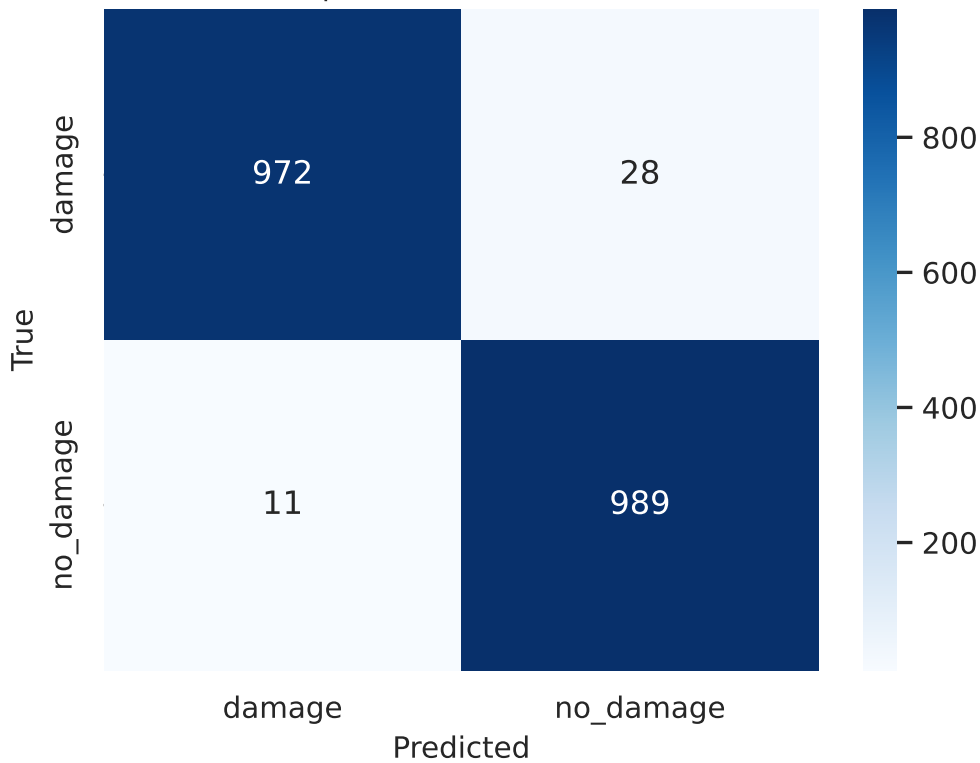
resnet34 | val Confusion (calibrated)
