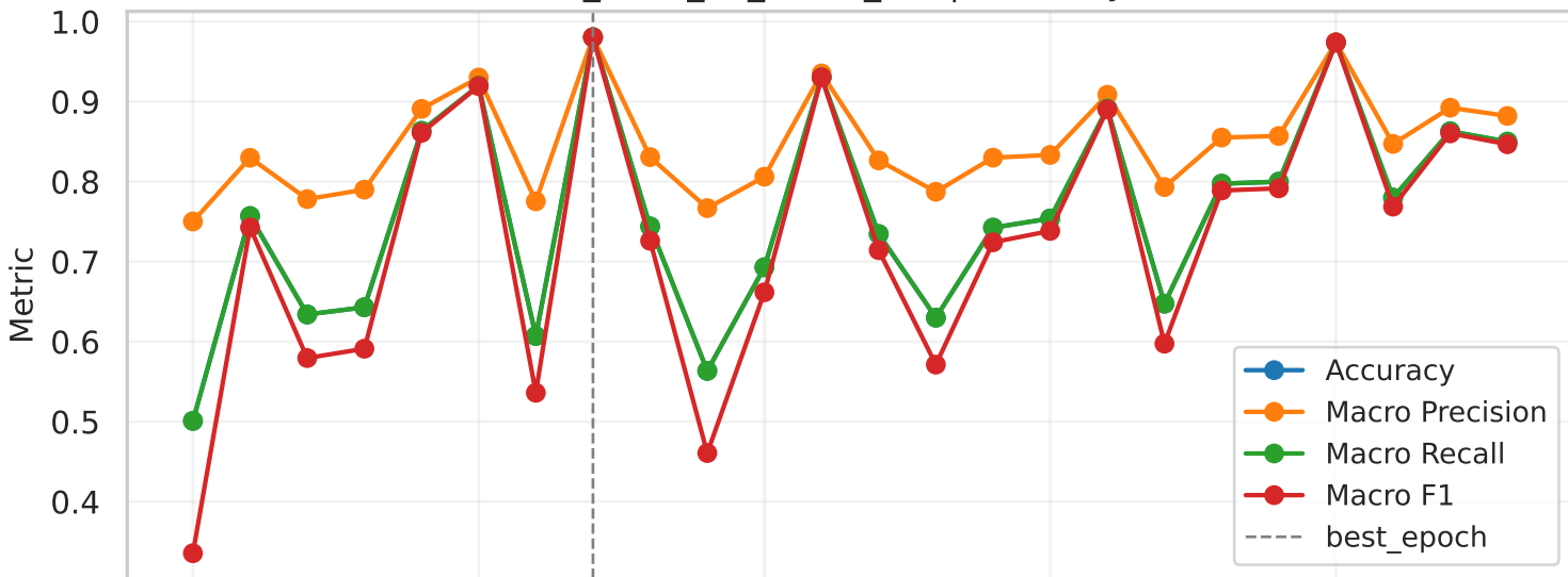
resnet34 (Run: data_2025_12_11-22_35) | Accuracy/Precision/Recall/F1
