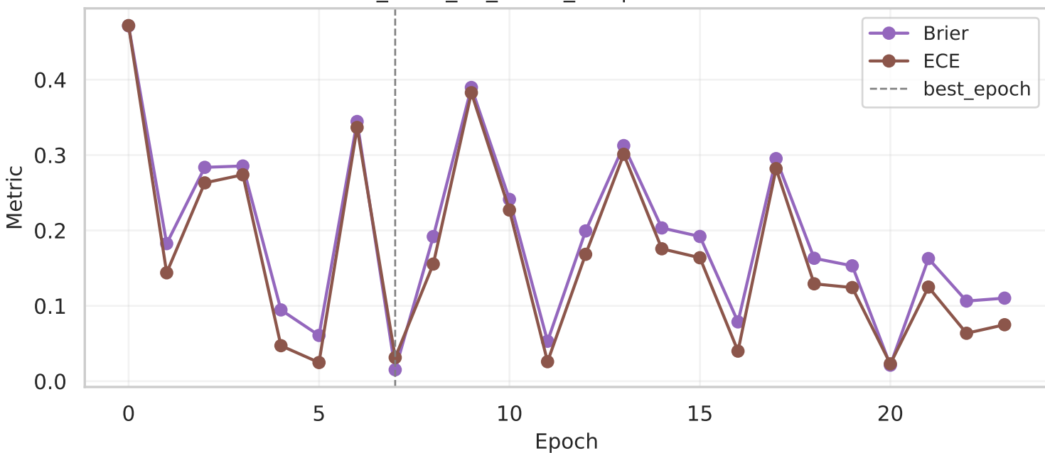
resnet34 (Run: data_2025_12_11-22_35) | Calibration metrics (Brier/ECE)
