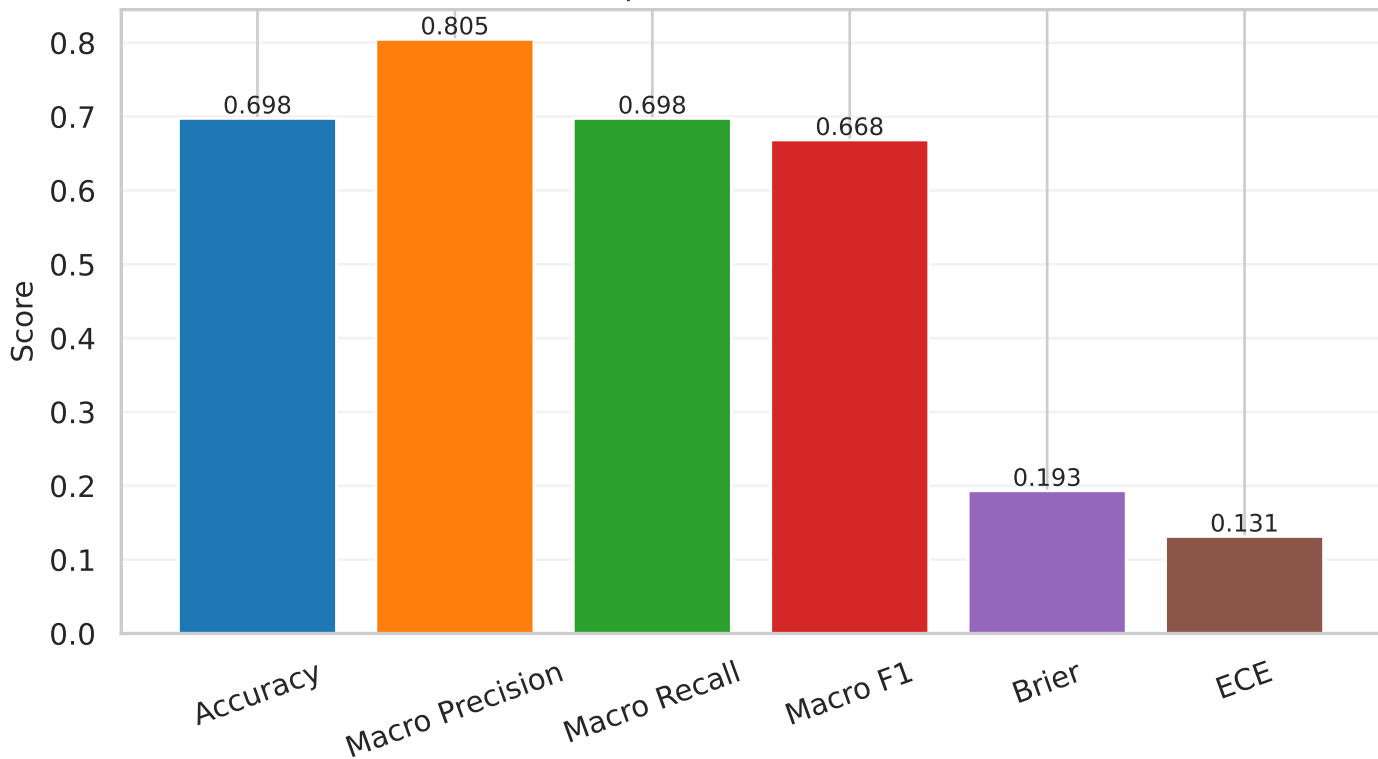
resnet50 | test (calibrated) metrics
