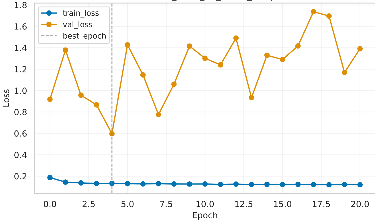
resnet50 (Run: data_2025_12_11-22_35) | Loss curves
