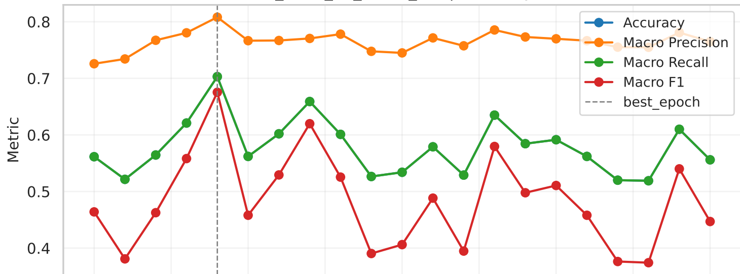
resnet50 (Run: data_2025_12_11-22_35) | Accuracy/Precision/Recall/F1
