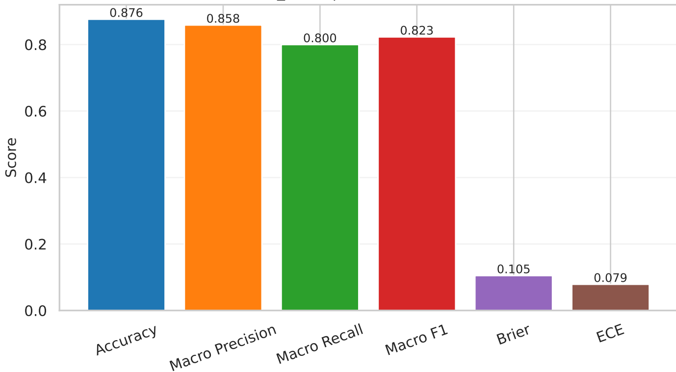
convnext_small | test (calibrated) metrics
