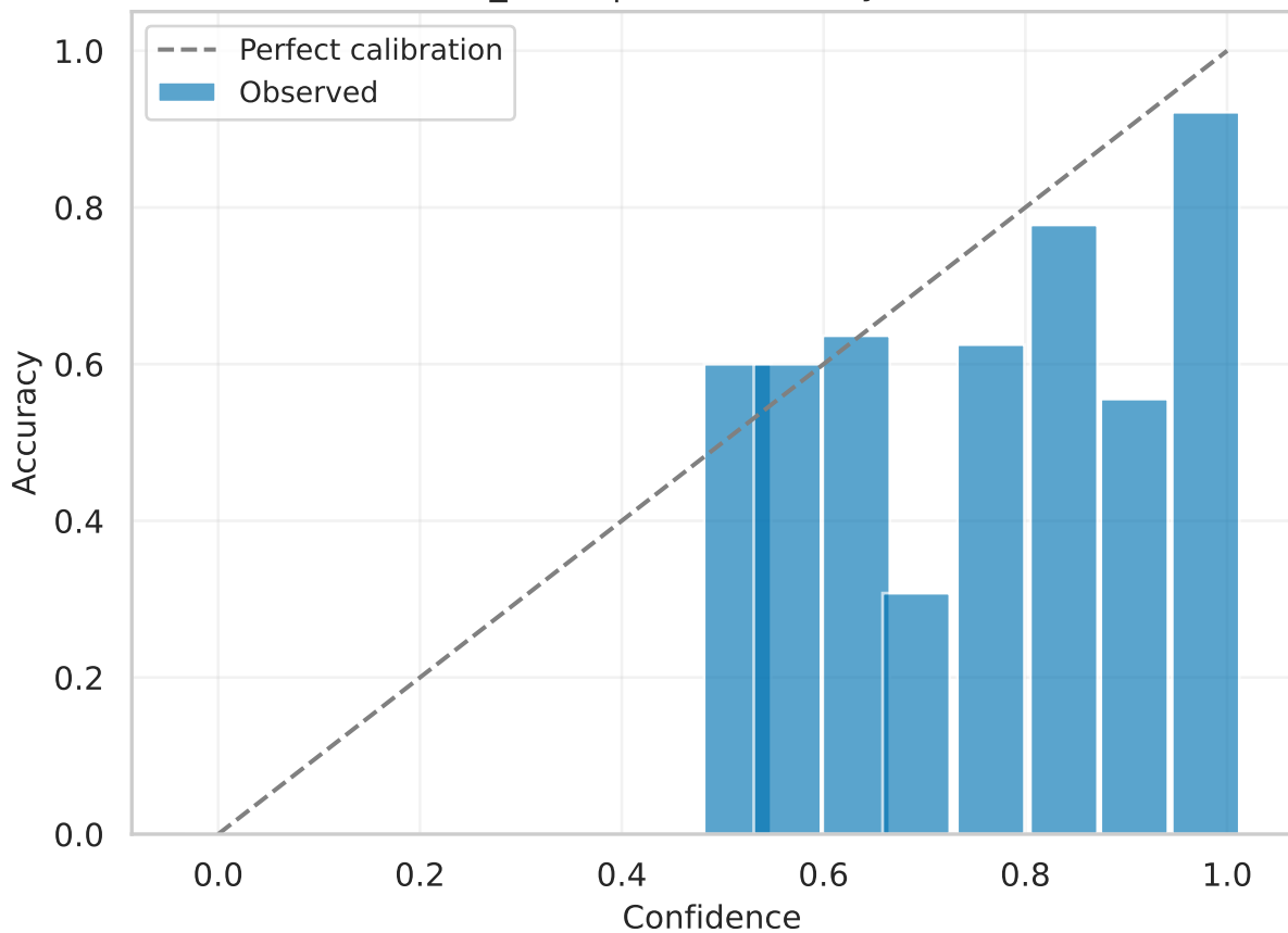
convnext_small | test Reliability (calibrated)
