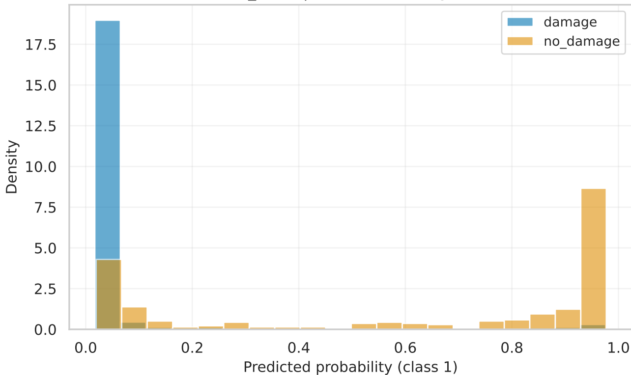
convnext_small | test Score Histogram (raw)
