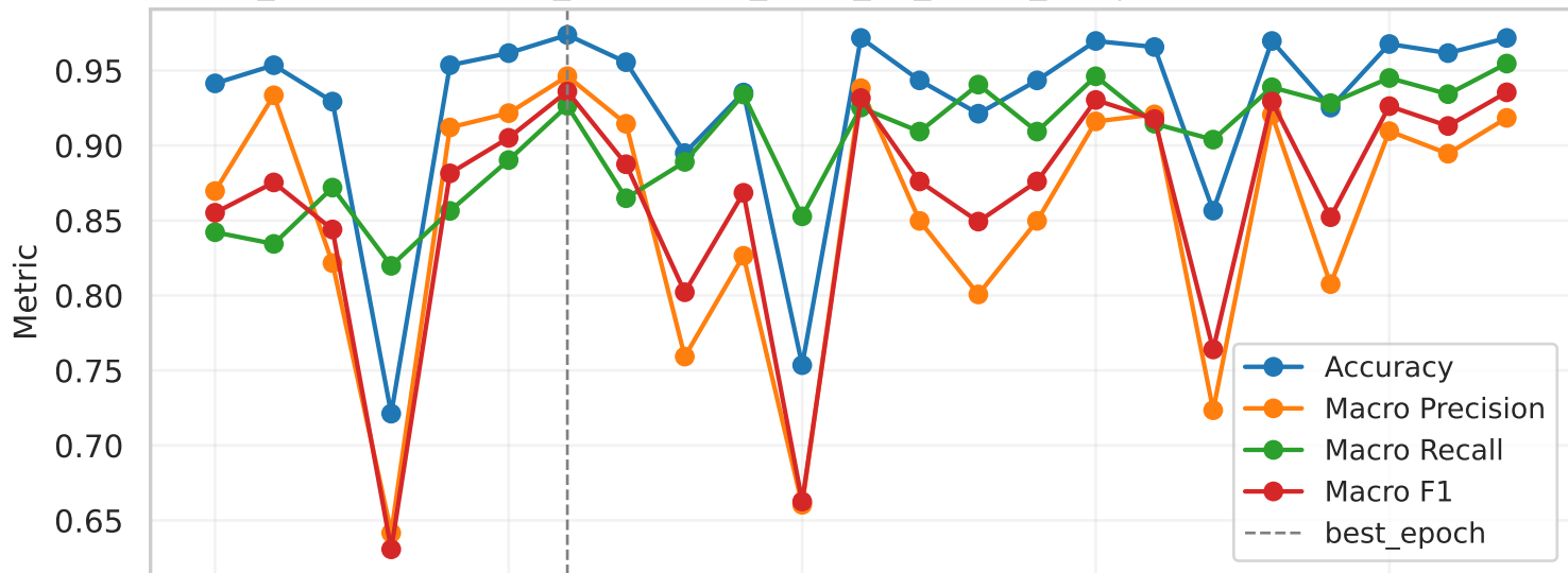
convnext_small (Run: data_resampled_2025_12_11-22_35) | Accuracy/Precision/Recall/F1
