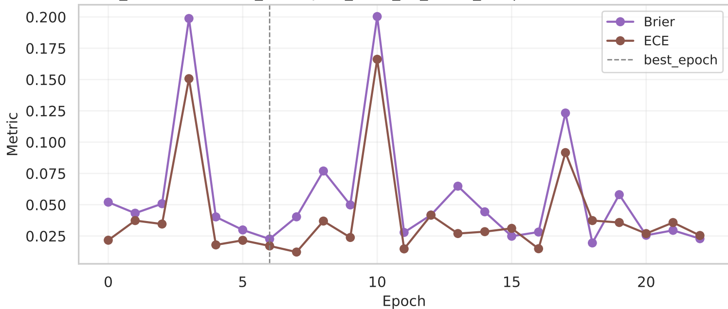
convnext_small (Run: data_resampled_2025_12_11-22_35) | Calibration metrics (Brier/ECE)
