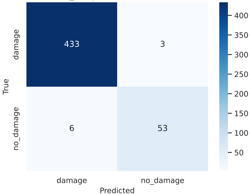
convnext_tiny | val Confusion (calibrated)
