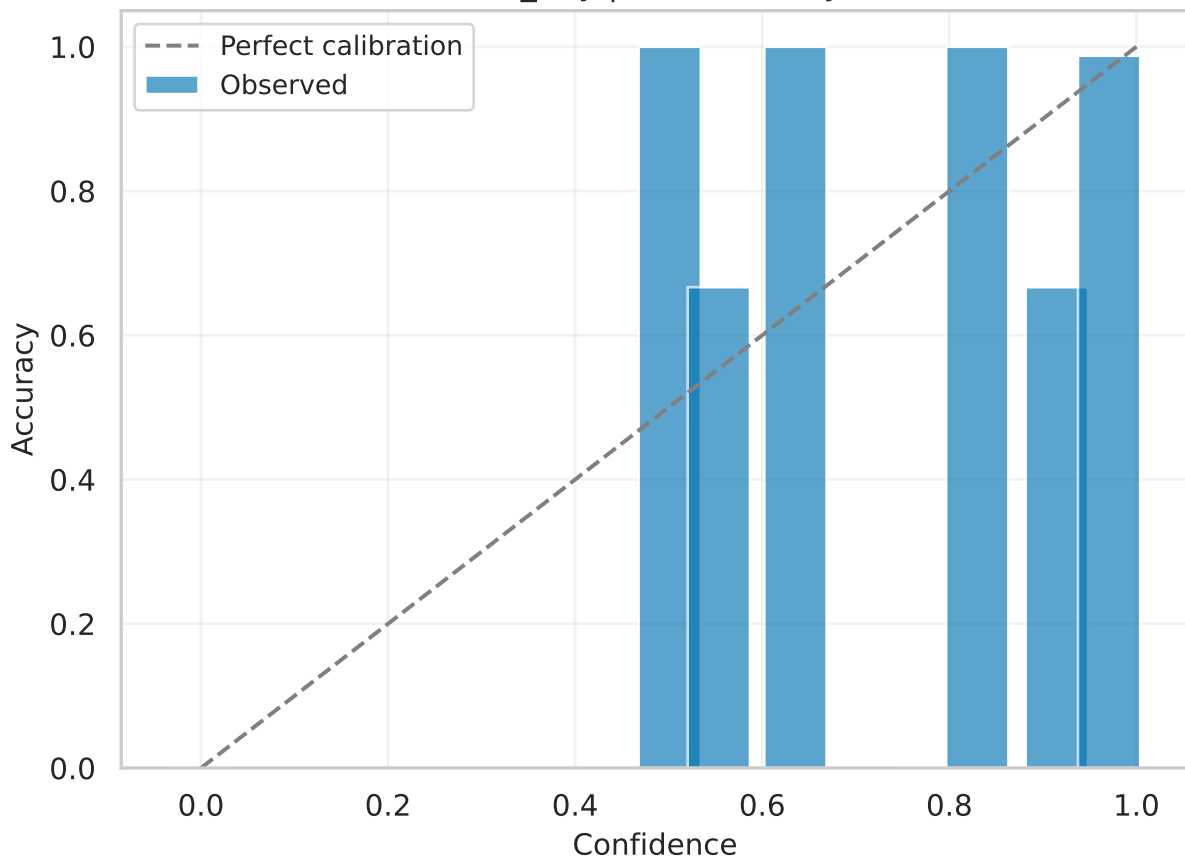
convnext_tiny | val Reliability (raw)
