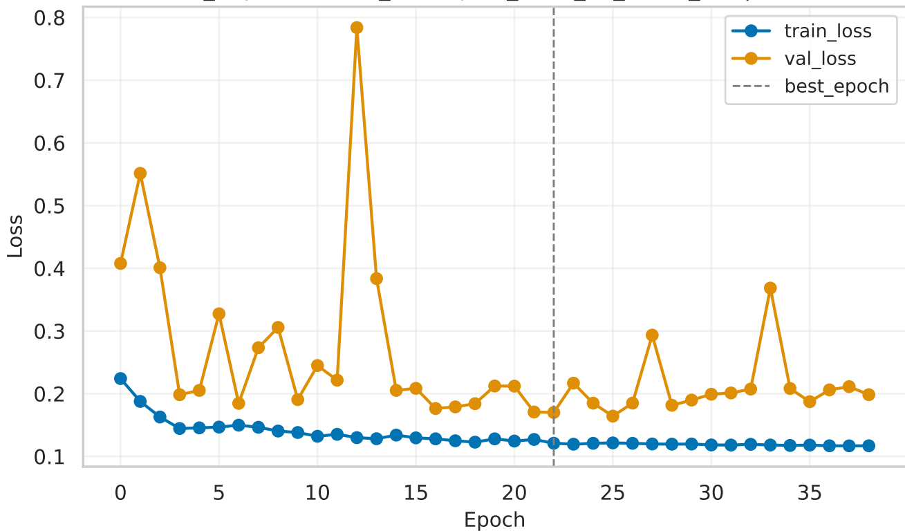
convnext_tiny (Run: data_resampled_2025_12_11-22_35) | Loss curves
