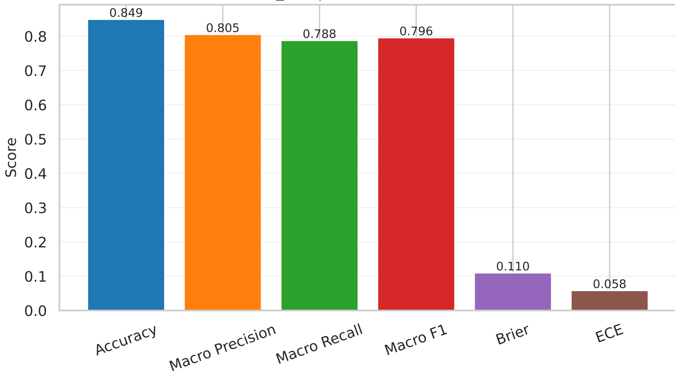
custom_cnn | test (calibrated) metrics
