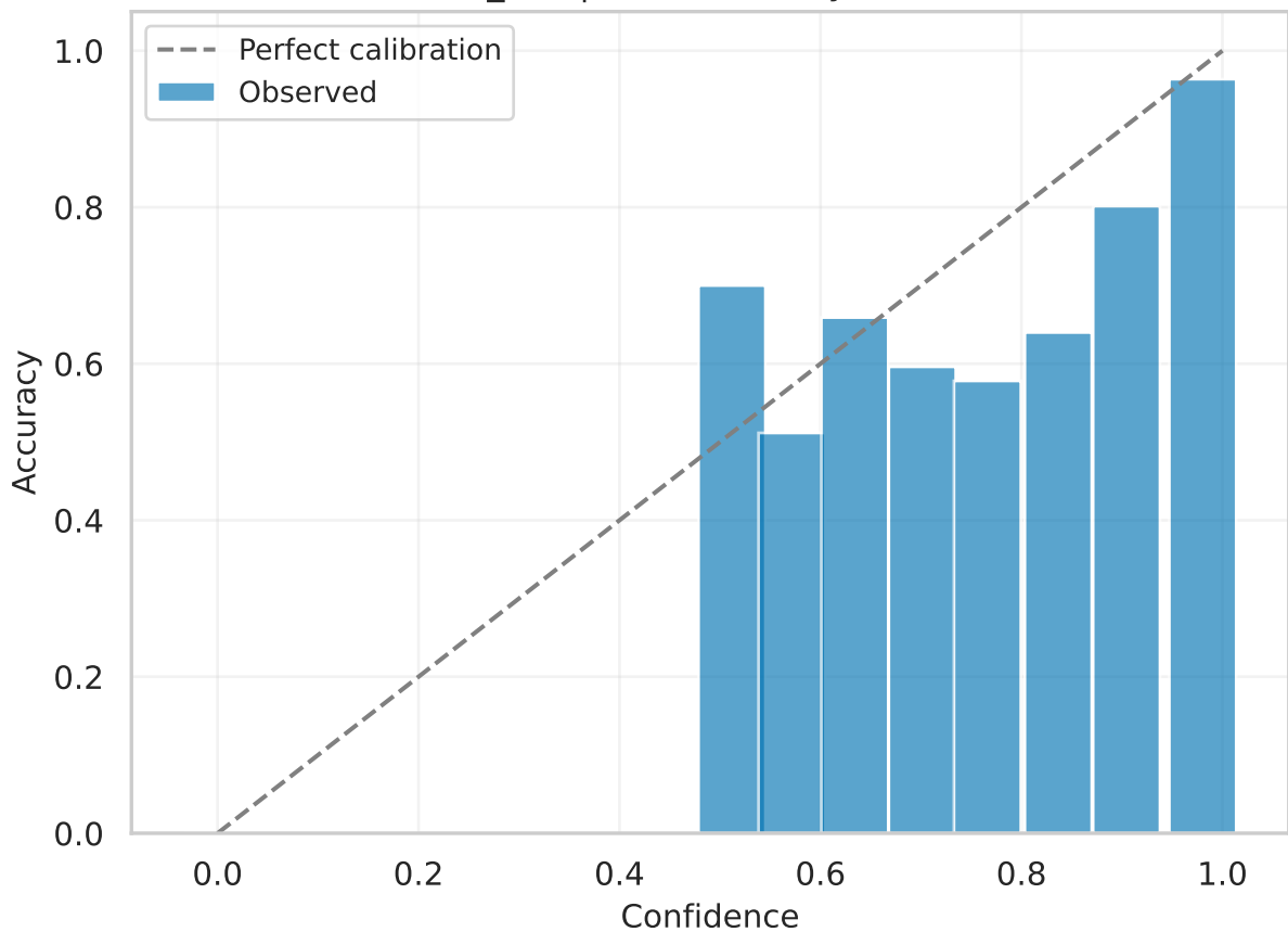
custom_cnn | test Reliability (calibrated)
