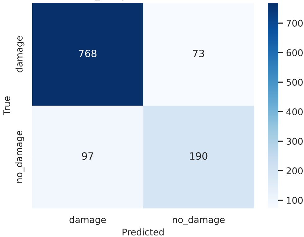
custom_cnn | test Confusion (raw)
