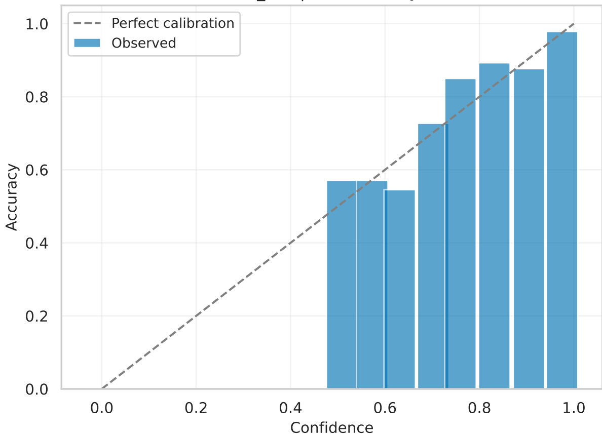
custom_cnn | val Reliability (raw)
