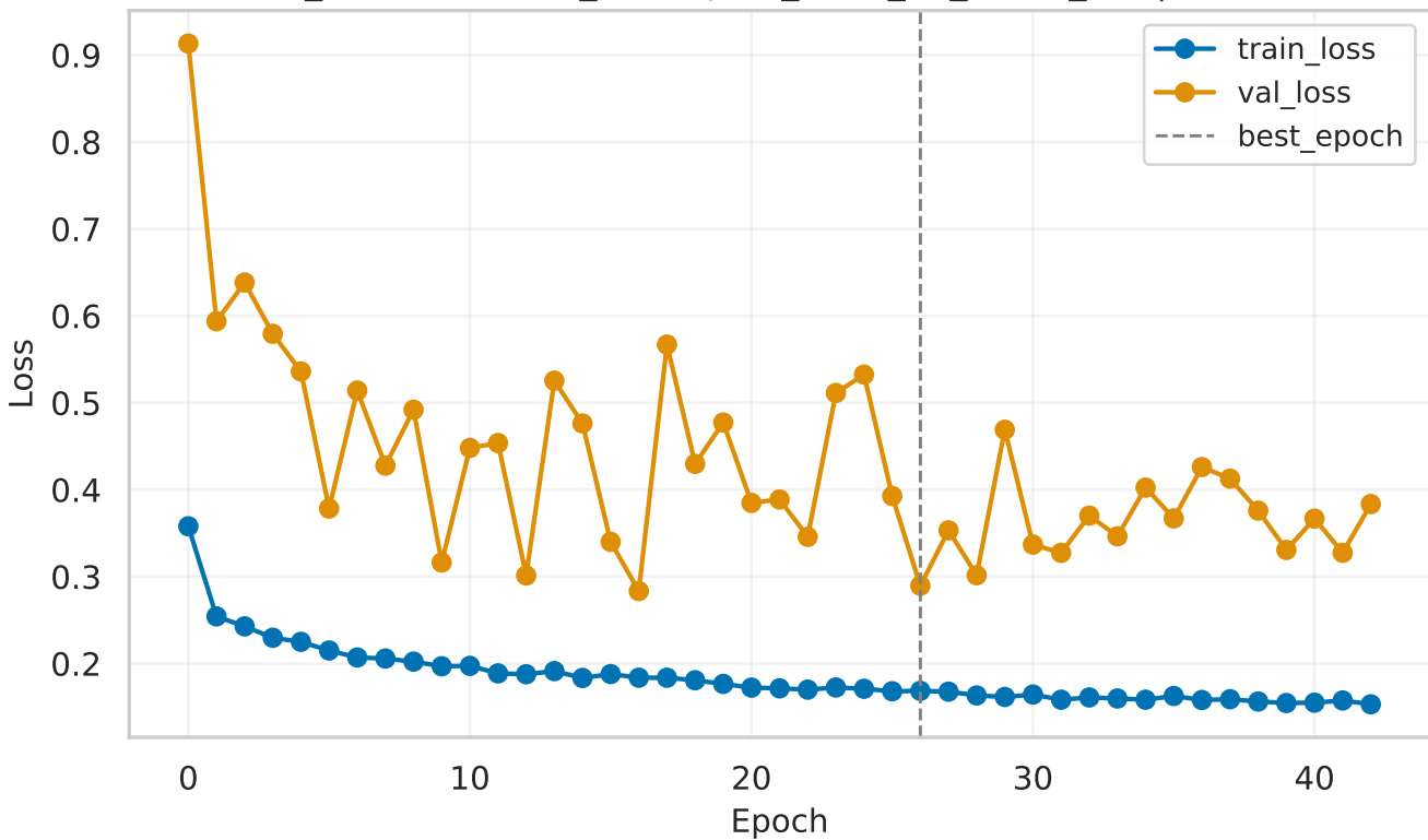
custom_cnn (Run: data_resampled_2025_12_11-22_35) | Loss curves
